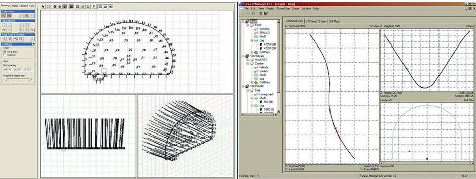
Figure 1 Underground Manager, software user interface. (Source: Adapted from Atlas Copco Rock Drills AB – Underground Rock Excavation Division, 2012).
